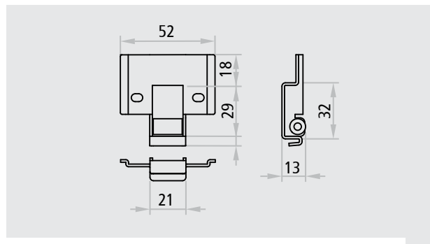
Upper strike box for inactive leaf of PROGET and other multipurpose doors
