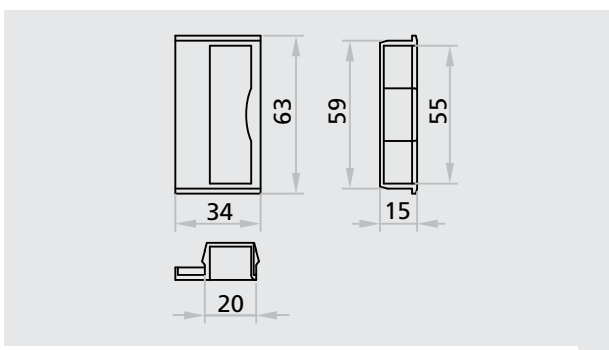
Strike box lock insert for one-leaved doors of PROGET and other multipurpose doors
