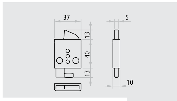
Upper re-latch device for inactive leaf of UNIVER and REVER
