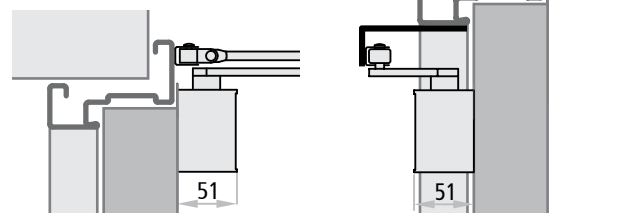
CP1 PROGET (from pull side) CP1-G PROGET (from push side)
