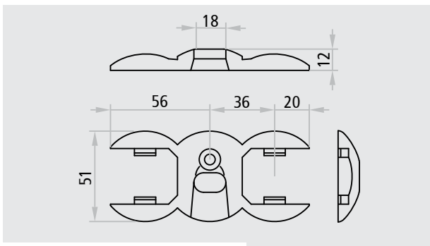
Lower floor catch for inactive leaf of REVER
