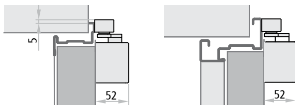
CP2 UNIVER CP2 PROGET
