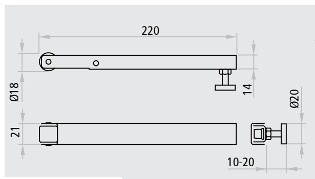
Carrier arm for inactive leaf
