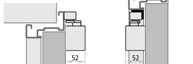
CP2 PROGET (from pull side) CP2-G PROGET (from push side)
